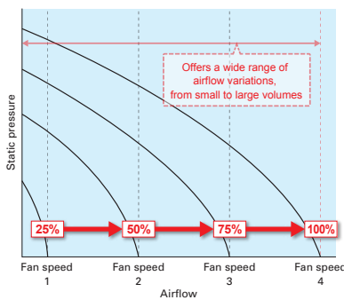
■ Characteristic curves of the LGH-RVX/RVXT Series
